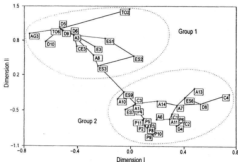
Fig. 3 Bidimensional representation of multidimensional scaling (MDS) with superimposed minimum spanning tree (MST) based on standard genetic distances (Nei 1978) between all sample pairs of brown trout analysed in Duero Basin. The MDS showed an excellent fit to original distances (stress = 0.05). The NTSYS package (Rohlf 1992) was used to conduct this ordination analysis. See Table 1 for population codes.
