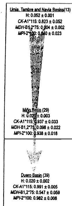
Fig. 4 Clinal variation of the mean gene frequency ( \pm error) for CK-A1*115, MPI-2*100 and sMDH-B1,2*75 alleles and of the mean intrapopulation genetic diversity ( H ) in native brown trout from the Iberian Peninsula around the 42° N parallel. In parentheses are the numbers of populations analysed in each group. Data of native nonisolated populations from Navia, Tambre, Umia, and Miño Basins were taken from Bouza et al. (1999) and Martínez et al. (1993).
