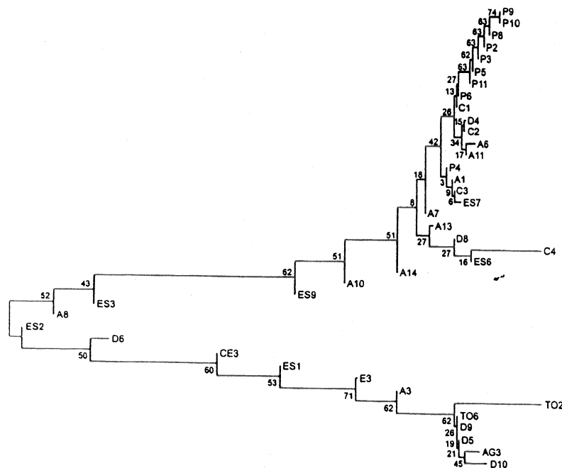
Fig. 2 Genetic relationships among 39 populations of brown trout sampled in Duero Basin obtained by the neighbour-joining (NJ) algorithm (Saitou & Nei 1987) from standard genetic distances (Nei 1978) between all sample pairs analysed. Branch lengths are proportional to the amount of change and NJ bootstrap values are based on 1000 replicates. The DISPAN program was used to carry out this analysis. See Table 1 for population codes.
